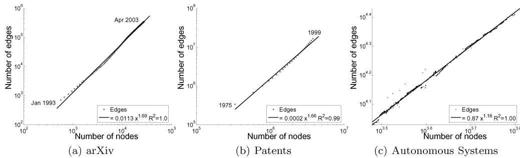
Fig. 5. The Densification Power Law. The number of edges E(t) is plotted against the number of nodes N(t) on log-log scales for (a) the arXiv citation graph, (b) the patents citation graph, and (c) the Internet Autonomous Systems graph. All of these grow over time, and the growth follows a power law in all three cases [Leskovec et al. 2005].
