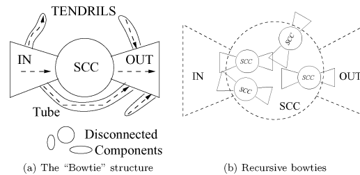
Fig. 7. The bowtie structure of the Web: Plot (a) shows the 4 parts: IN, OUT, SCC, and TENDRILS [Broder et al. 2000]. Plot (b) shows recursive bowties: sub-graphs of the WWW can each be considered a bowtie. All these smaller bowties are connected by the navigational backbone of the main SCC of the Web [Dill et al. 2001].
