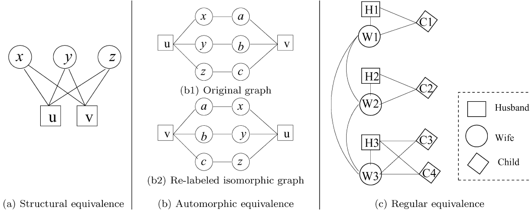
Fig. 19. Social roles and equivalences. (a) Nodes u and v are structurally equivalent because they are linked to exactly the same set of nodes: x , y , and z . (b) Nodes u and v of plot (b1) are automorphically equivalent because we can exchange their positions, and then relabel the rest of the nodes as in plot (b2) so that the new graph is isomorphic to the original. (c) The squares (husbands), circles (wives) and rhombuses (children) form three regularly-equivalent classes. A husband connects to a wife and a child; a wife to a husband, child, and other wives; a child connects to a husband and a wife. Thus, each class is defined by its set of relationships to the other classes. Note that child C1 and C4 are not structurally or automorphically equivalent, but they are regularly equivalent.
