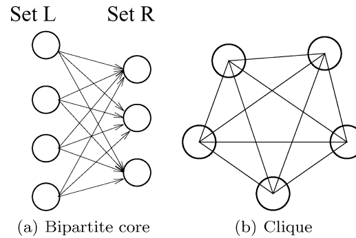
Fig. 4. Indicators of community structure. Plot (a) shows a 4 \times 3 bipartite core with each node in Set L being connected to each node in Set R . Plot (b) shows a 5-node clique where each node is connected to every other node in the clique.
