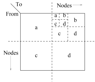
Fig. 15. The R-MAT model. The adjacency matrix is broken into four equal-sized partitions, and one of those four is chosen according to a (possibly nonuniform) probability distribution. This partition is then split recursively until we reach a single cell, where an edge is placed. Multiple such edge placements are used to generate the full synthetic graph.
