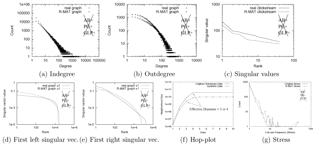
Fig. 18. Clickstream bipartite graph. The AB+ , PG+ and GLP+ methods do not apply . The crosses and dashed lines represent the R-MAT generated graphs, while the pluses and strong lines represent the real graph.
