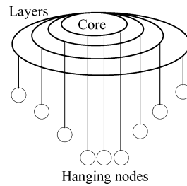
Fig. 6. The Internet as a Jellyfish. The Internet AS-level graph can be thought of as a core, surrounded by concentric layers around the core. There are many one-degree nodes that hang off the core and each of the layers.
