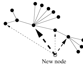
Fig. 10. The Barabási-Albert model. New nodes are added; each new node prefers to connect to existing nodes of high degree. The dashed lines show some possible edges for the new node, with thicker lines implying higher probability.
