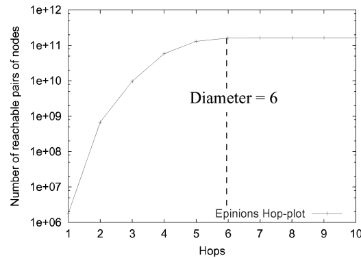
Fig. 2. Hop-plot and effective diameter. This is the hop-plot of the Epinions graph [Domingos and Richardson 2001; Chakrabarti et al. 2004]. We see that the number of reachable pairs of nodes flattens out at around 6 hops; thus the effective diameter of this graph is 6.
