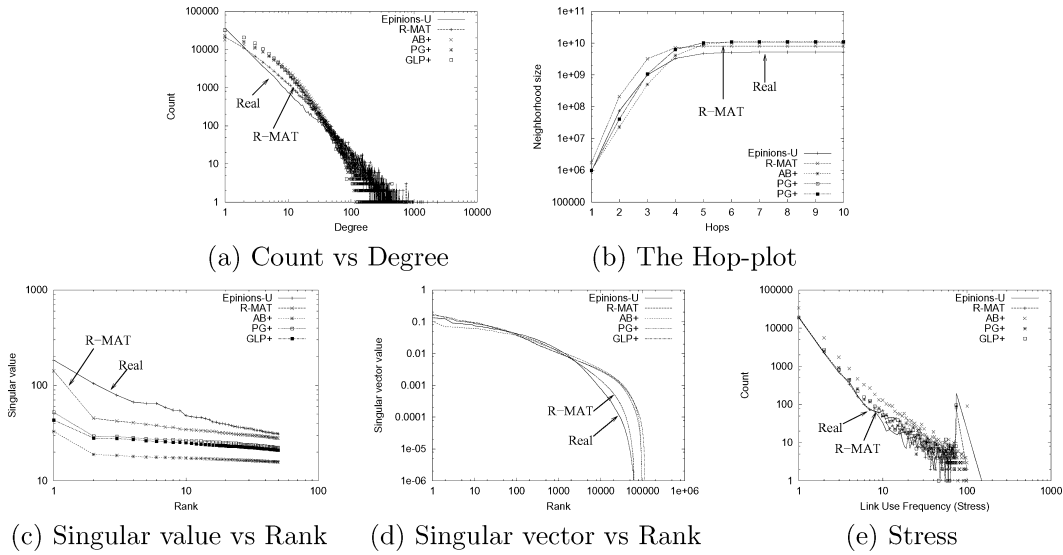
Fig. 16. Epinions-U undirected graph. We show (a) degree, (b) hop-plot, (c) singular value, (d) singular vector value, and (e) stress distributions for the Epinions-U dataset. R-MAT gives the best matches to the Epinions-U graph among all the generators. In fact, for the stress distribution, the R-MAT and Epinions-U plots are almost indistinguishable.
